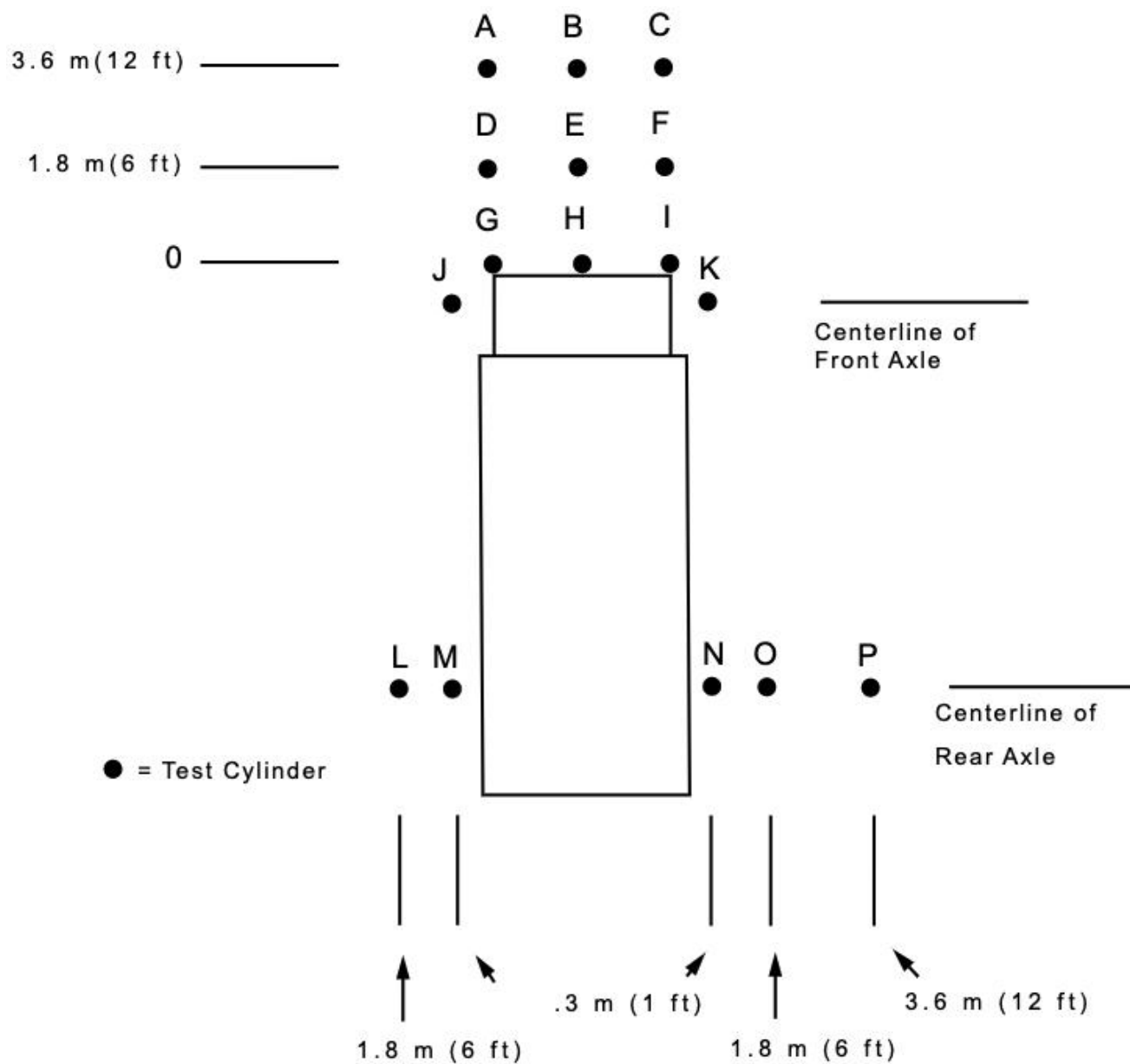
Figure 1 – Mirror Adjustment
