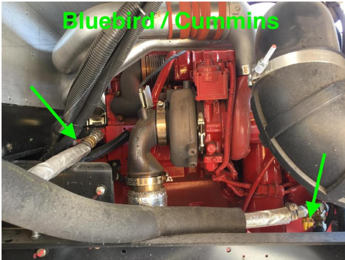
Figure 12 – Bluebird Cummins Heater Valves
